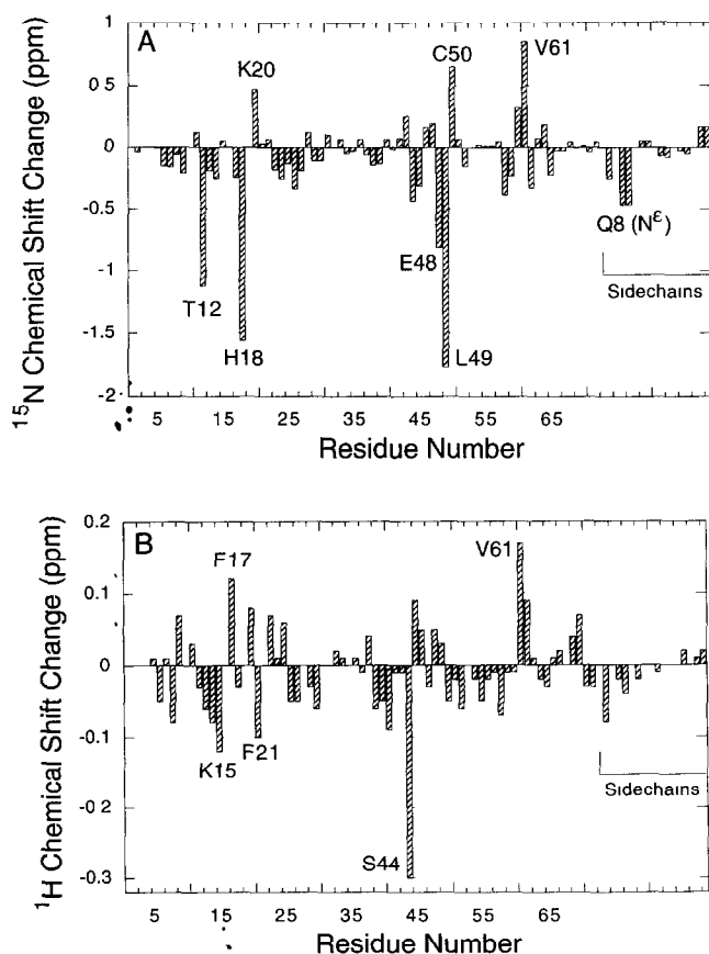
Fig. 3. (A) 15 N and (B) 1 H chemical shift differences between the 1 H- 15 N HSQC spectra of unligated IL-8 and the IL-8:IL8-r1 complex versus sequence number. Excluded resonances are overlapped in the 1 H- 15 N HSQC spectra. The ratio of IL8-r1 peptide to IL-8 monomer is 1.25:1 in the complex.
